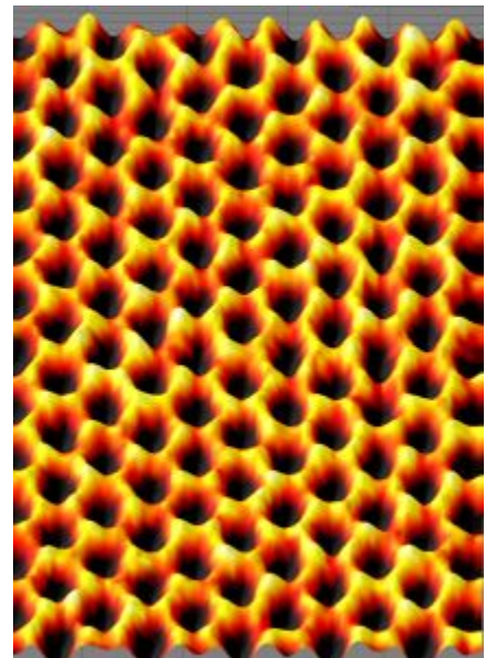
This image of a single suspended sheet of graphene taken with Transmission Electron Aberration-corrected Microscope shows individual carbon atoms (yellow) on the honeycomb lattice. (Image Source: Lawrence Berkley National Lab)
